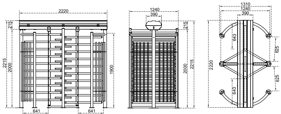
Dimensions (mm)
